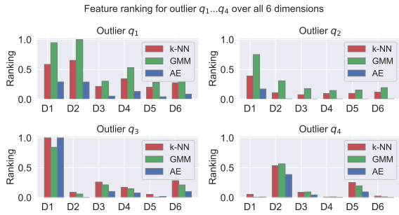
Figure 5: Feature ranking of the introduced outliers over all 6-dimensions for the three approaches scaled into the common range of [0, 1] .
