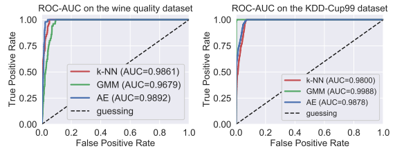
Figure 3: ROC-AUC of the different methods on the wine quality data set (left) and the KDD-Cup99 data set (right).
