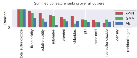
Figure 7: Wine Quality data set: Summed-up feature ranking of the outliers (red wine) over all 6-dimensions for the three approaches scaled into the common range of [0, 1] .
