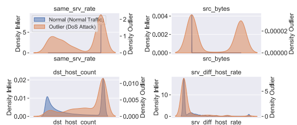
Figure 12: KDD-Cup99 data set: Density estimation of the top 4 features for the outliers (attack) and normal instances.
