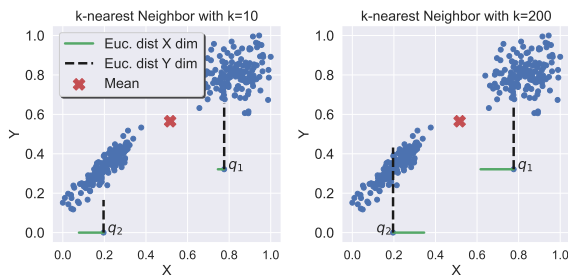
Figure 1: Feature ranking: Mean Euclidean distance per dimension for two selected outliers with k = 10 (left) and a too large value of k = 200 (right).
