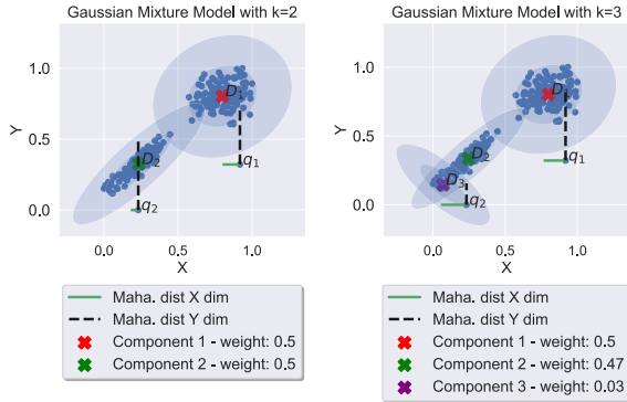
Figure 2: Mahalanobis distance per dimension for two selected outliers as explanation. On the left a GMM with k = 2 and on the right a GMM with k = 3 is fitted on the data
