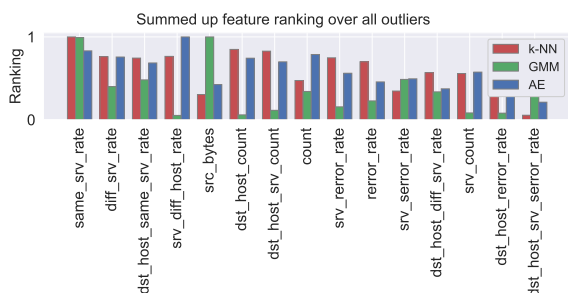
Figure 11: KDD-Cup99 data set: Feature ranking of the outliers over the top 15 dimensions for the three approaches scaled into the common range of [0, 1].
